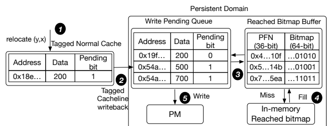
Figure 10: FFCCD design.
