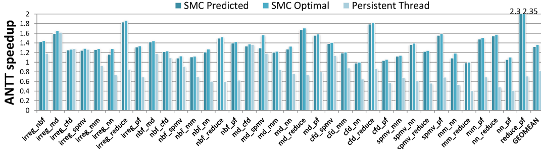
Figure 3: Speedup of average normalized turnaround time.
