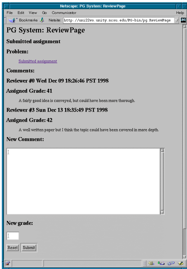
Figure 3: Review page
